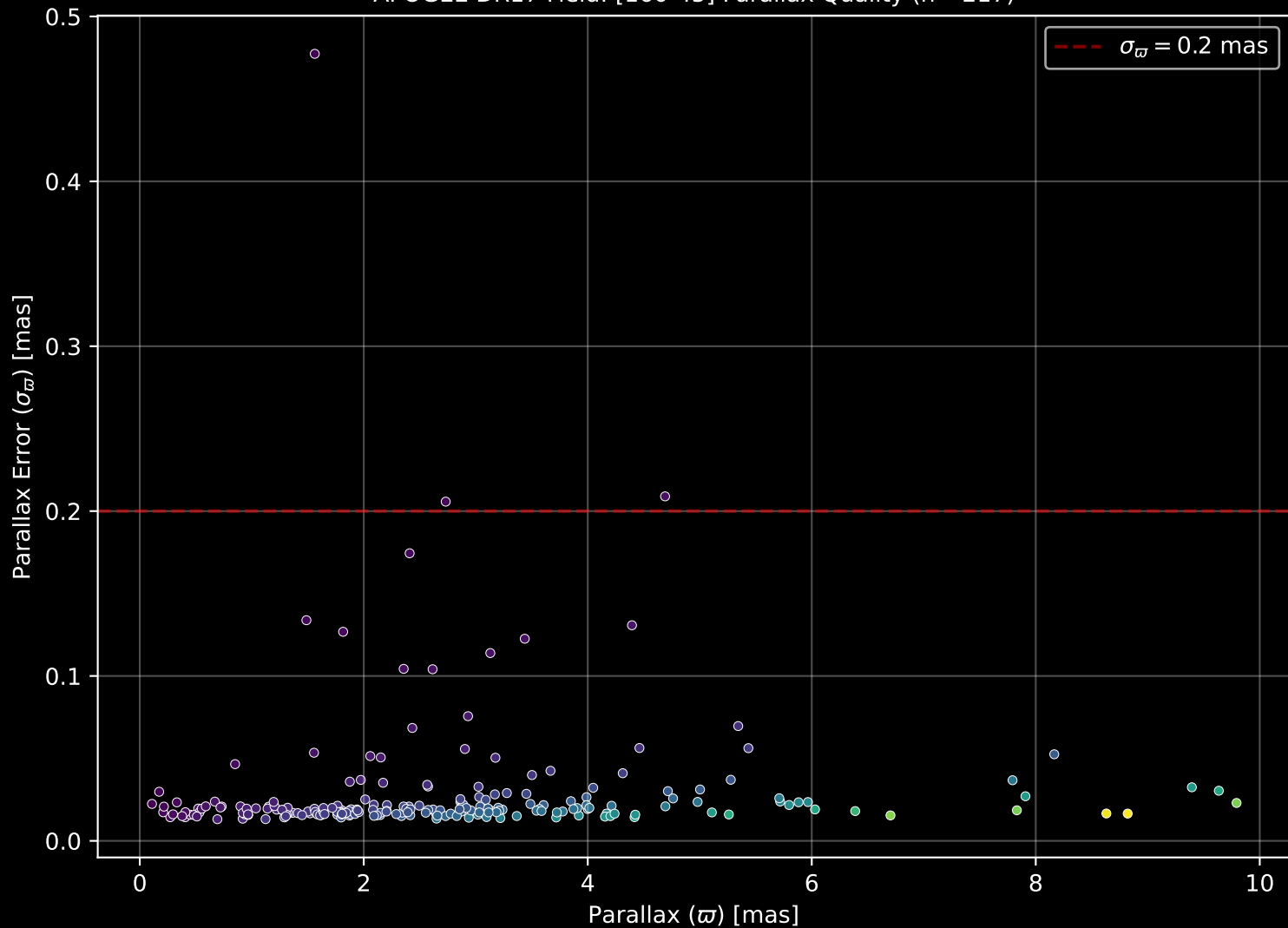
APOGEE DR17 Field: [160-45] Parallax Quality (n= 217)
