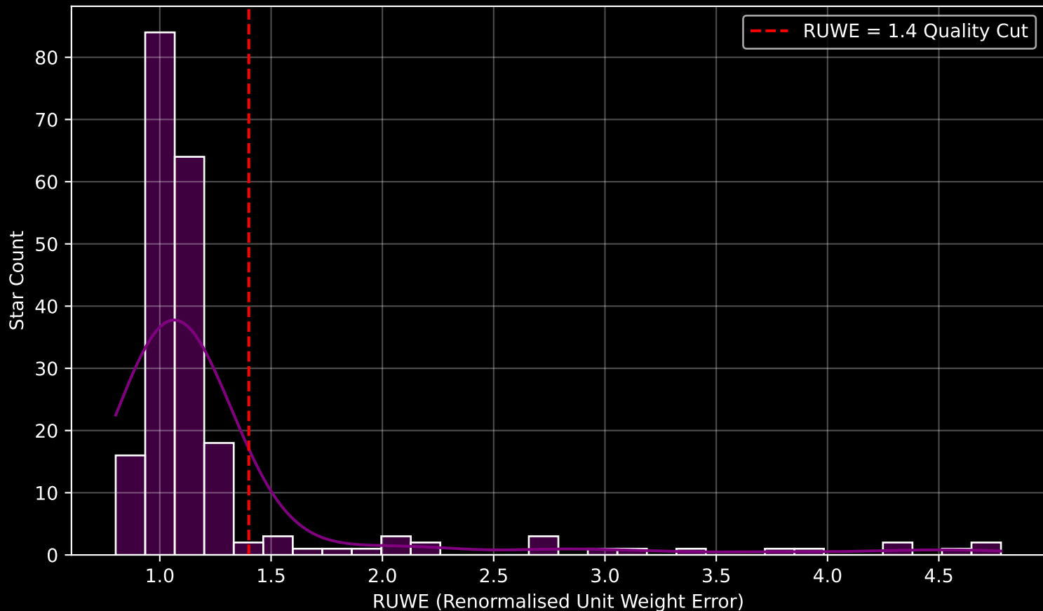
GAPOGEE DR17 Field [160-45] RUWE Distribution (n= 208)
