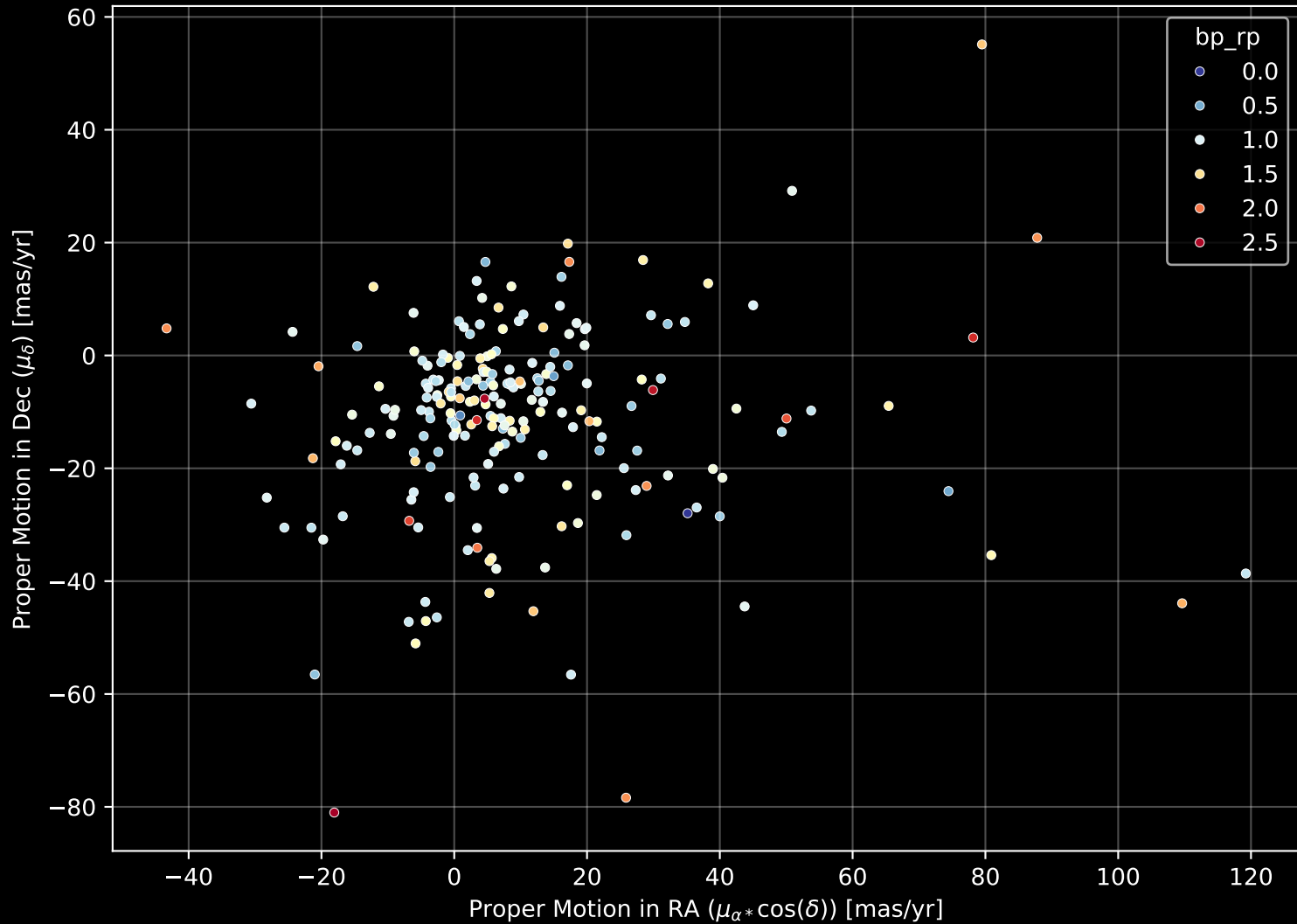
APOGEE DR17 Field: [160-45] Proper Motion Diagram (n= 217)
