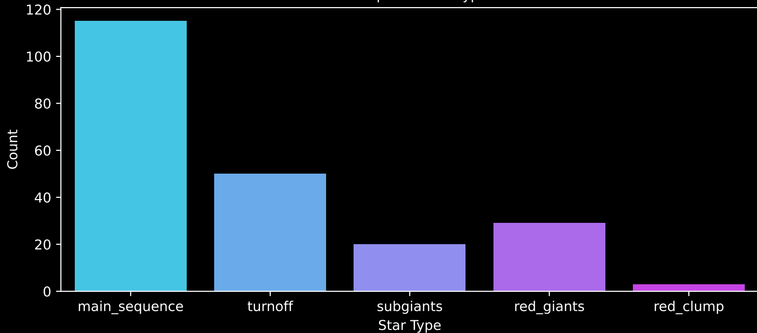
APOGEE DR17 Field: [160-45] Count plot of Star Type
