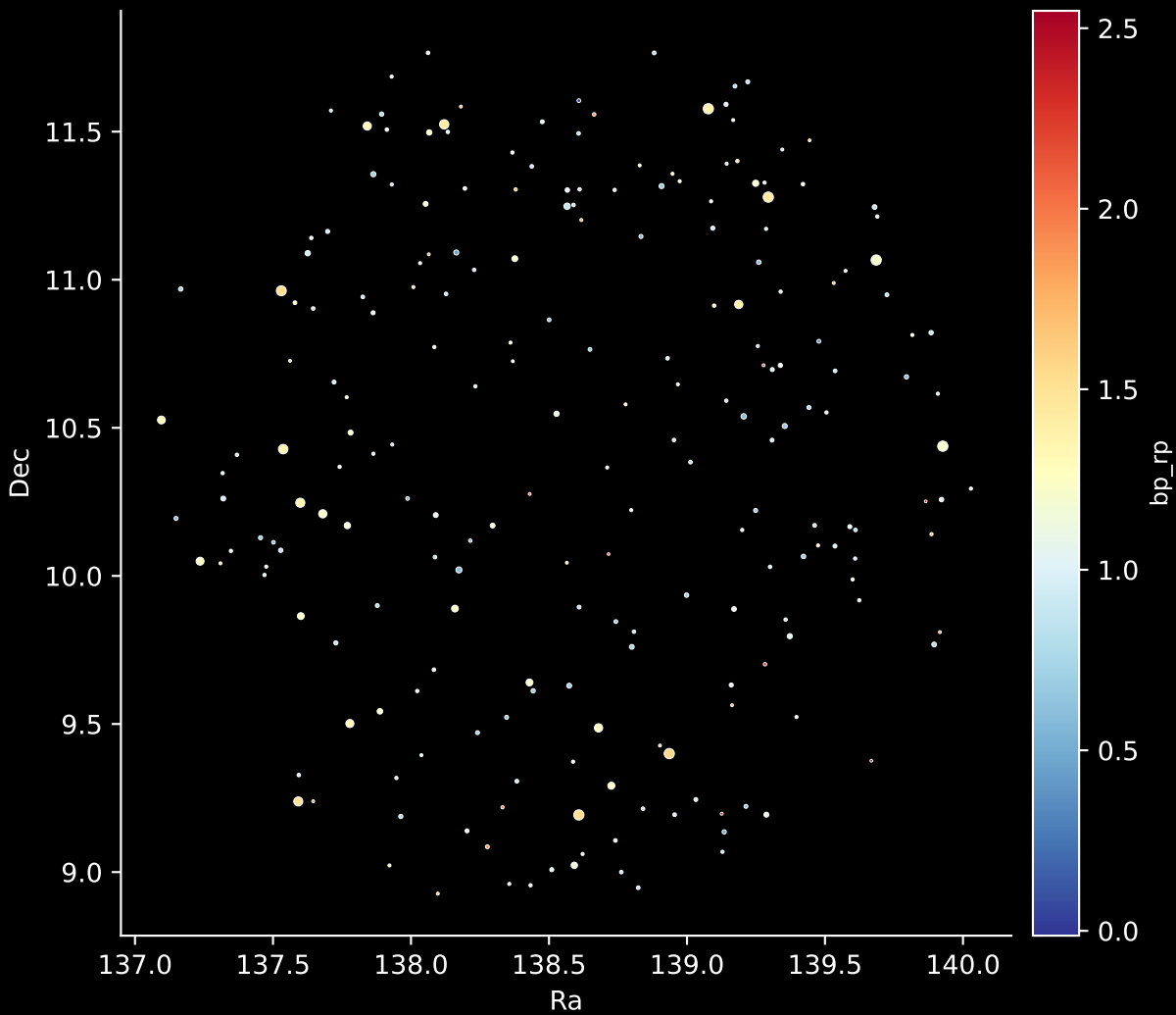
APOGEE DR17 Field: [160-45] Stars: 217
