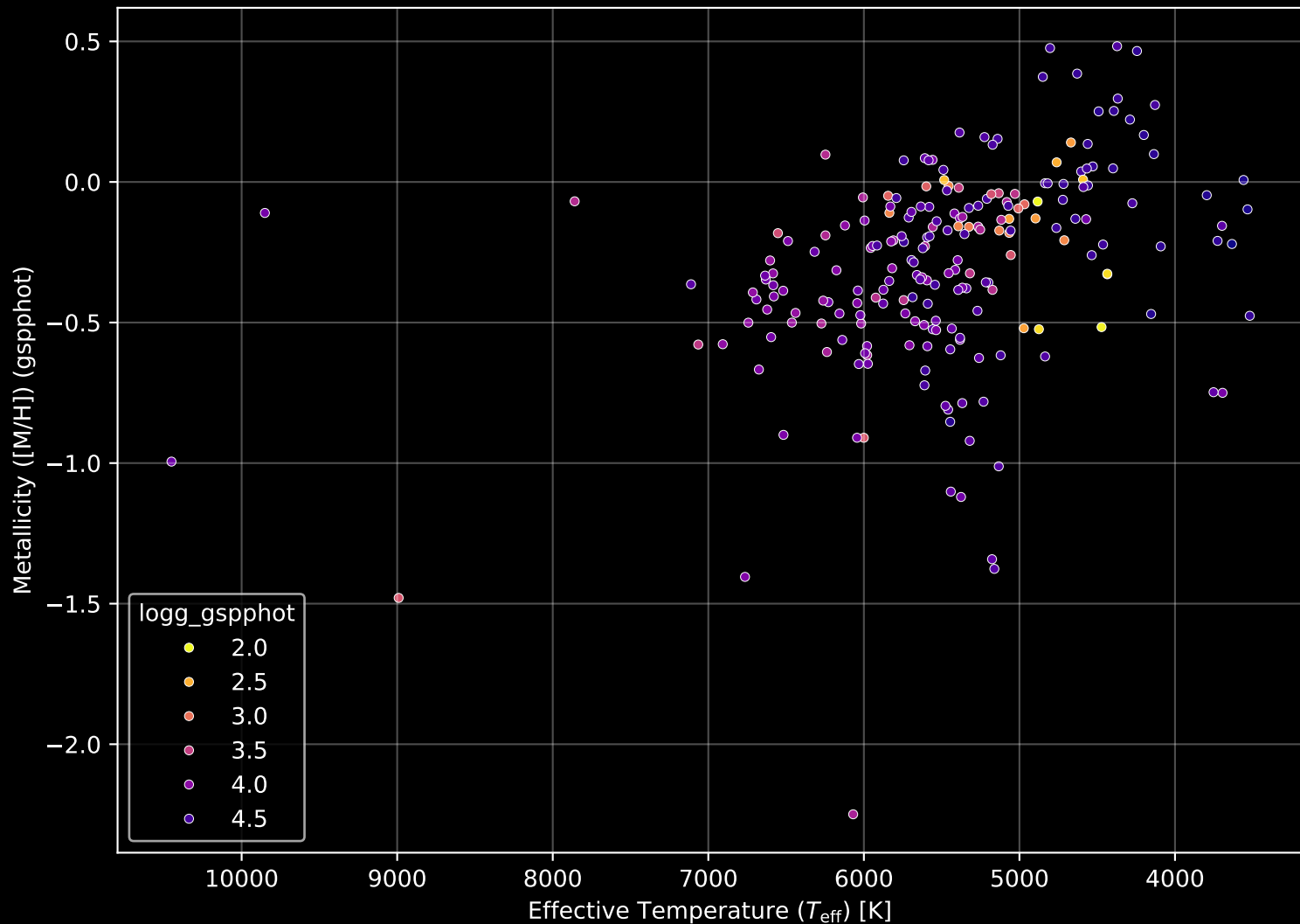
APOGEE DR17 Field: [160-45] Stellar Population Parameters (n= 217)
