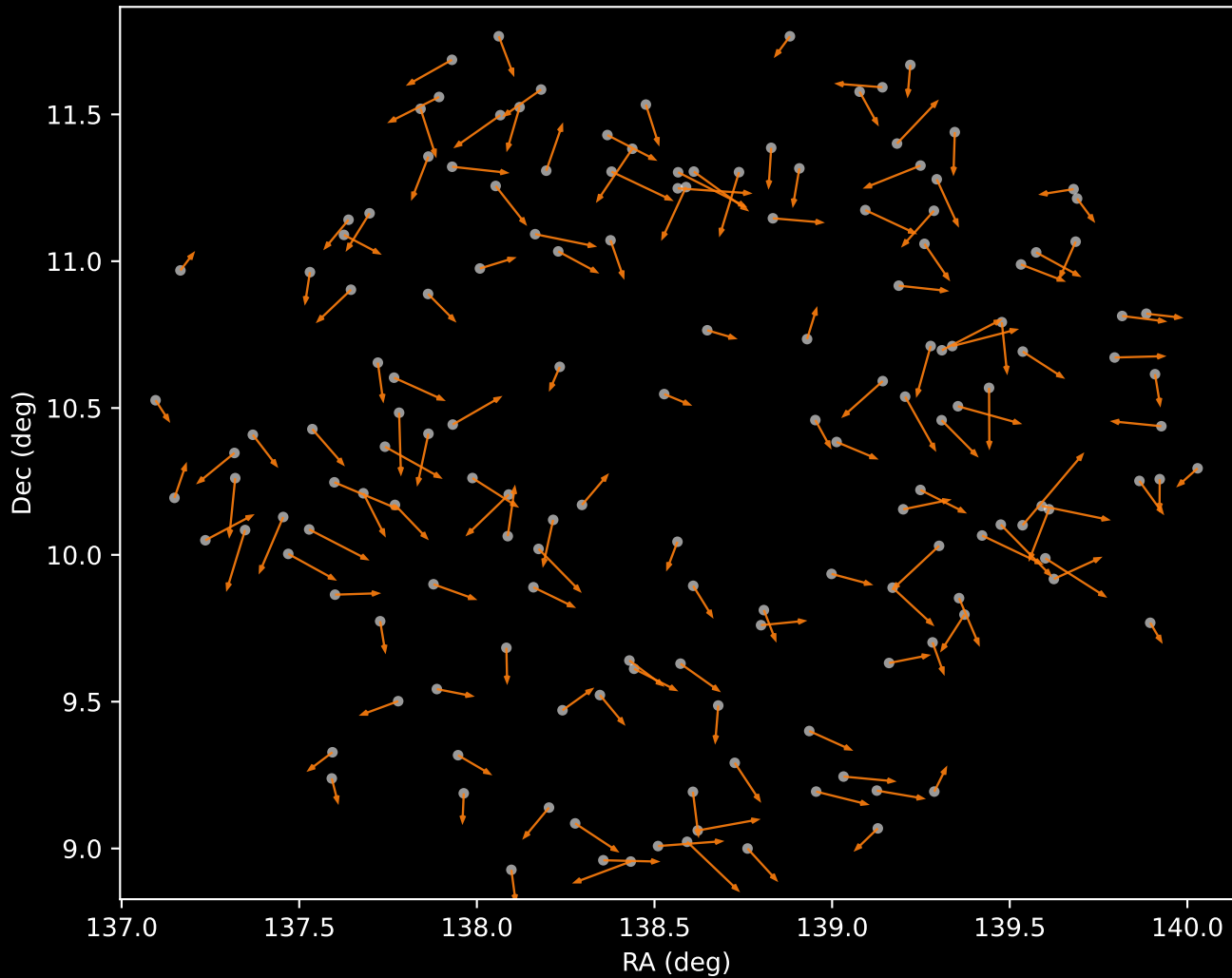
APOGEE DR17 Cluster 2 Proper Motion Vectors (n=156)
