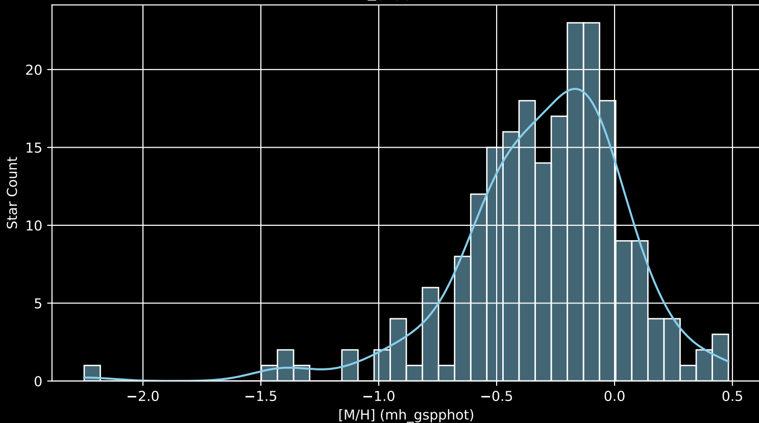
APOGEE DR17 Field: [160-45 [M/H] (mh_gspphot) (n= 217)
